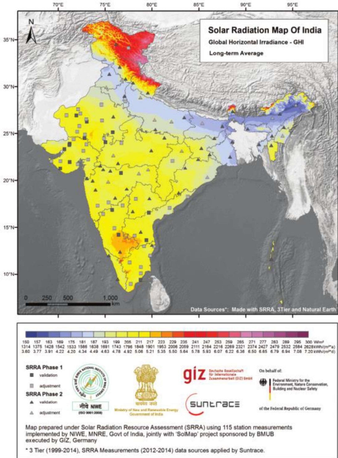
Fig A.2: SRRA Map GHI (Long Term Average)
