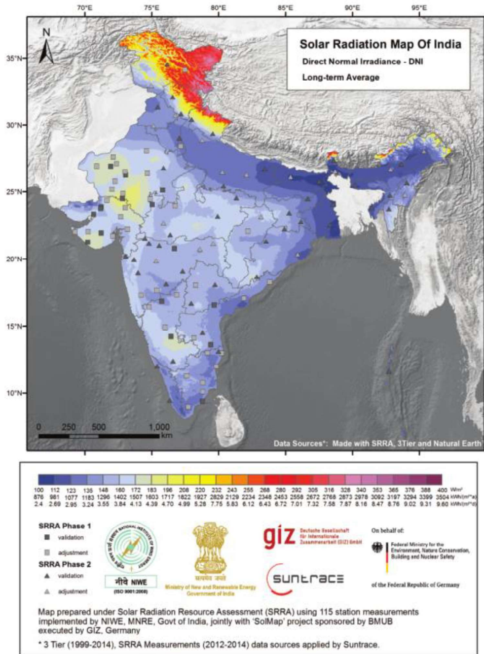
Fig A.1: SRRR Map DNI (Long Term Average)
