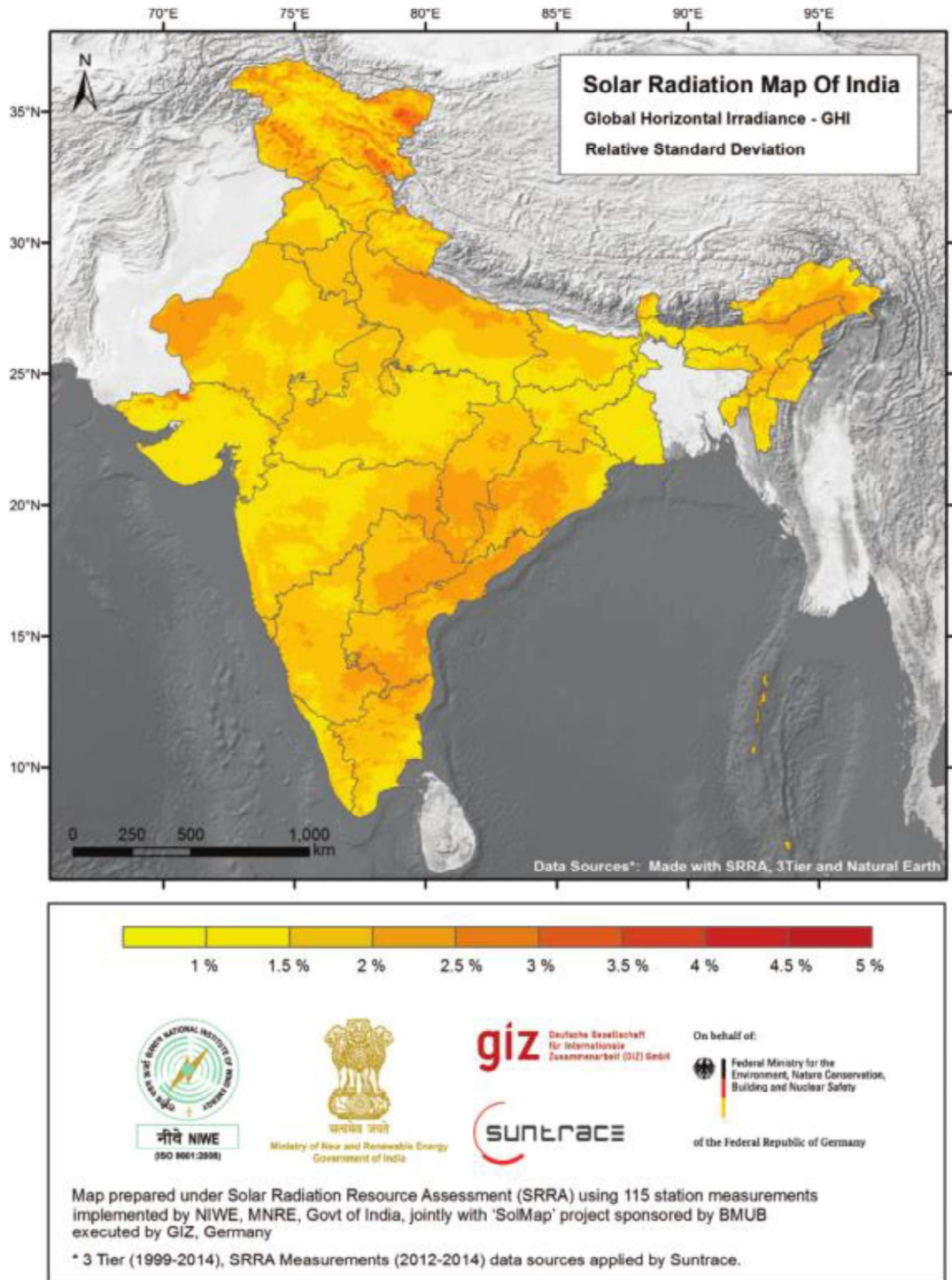
A.1.3: SRRA MAP GHI (RELATIVE STANDARD DEVIATION) [Source: C-WET, 2017]
