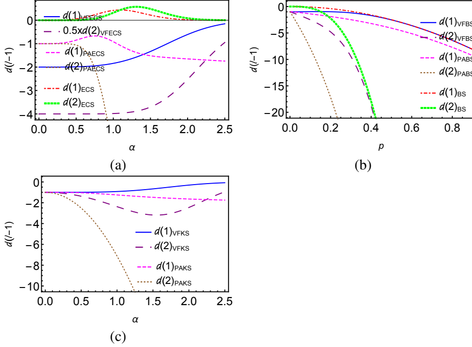
Figure 5.1: Lower- and higher-order antibunching witnesses as functions of displacement parameter \alpha (for ECS and KS) and probability p (for BS with parameter M = 10 ) for (a) ECS, PAECS and VFECs, (b) BS, PABS and VFBS, and (c) KS, PAKS and VFKS. The quantities shown in all the plots are dimensionless.
