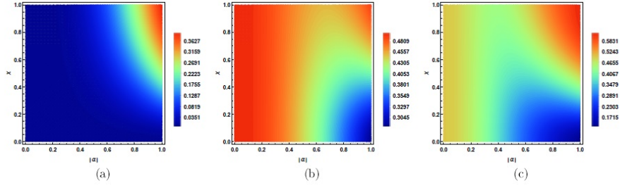
Figure 5.6: Illustration of linear entropy for (a) KS (b) VFKS (c) PAKS.
