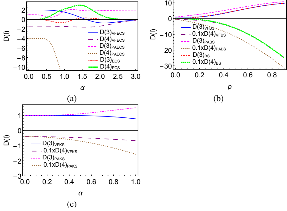
Figure 5.4: Illustration of HOSPS as a function of displacement parameter \alpha (for ECS and KS) and probability p (for BS) for (a) ECS, (b) BS, and (c) KS and corresponding engineered states. HOSPS is not observed in KS.
