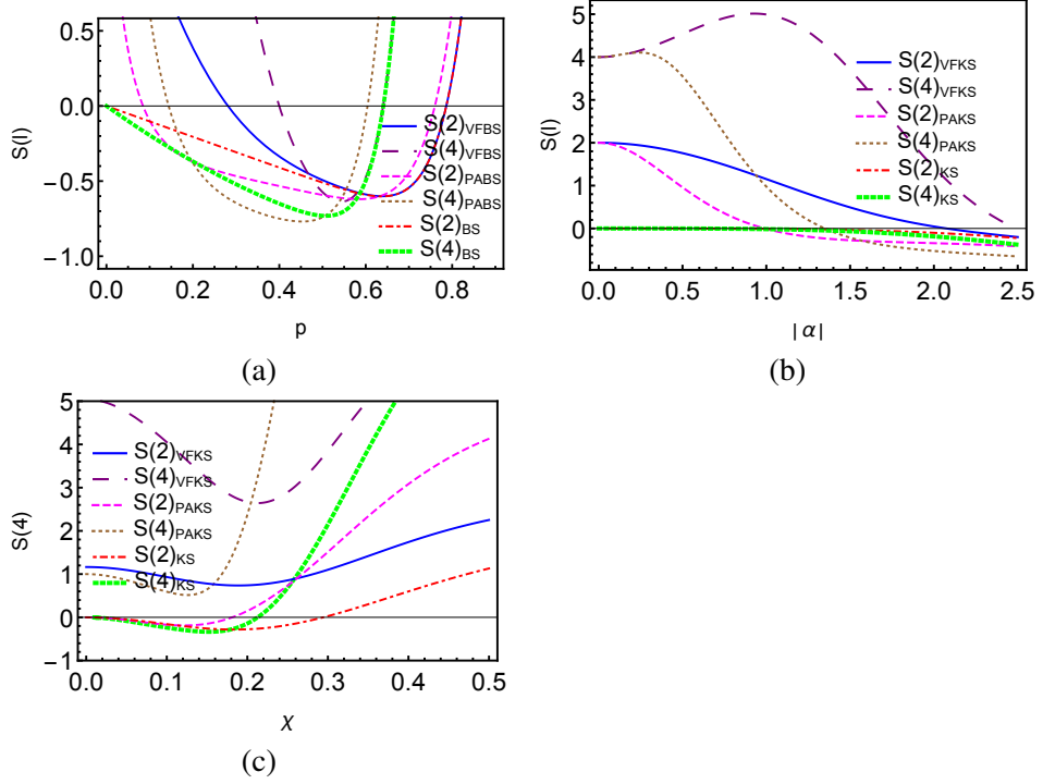
Figure 5.2: Illustration of lower- and higher-order squeezing for (a) BS, PABS and VFBS; (b) KS, PAKS and VFKS at the fixed value of \chi = 0.02 ; (c) KS, VFKS and PAKS as a function of \chi with \alpha = 1 . The negative regions of the curves illustrate the presence of squeezing.
