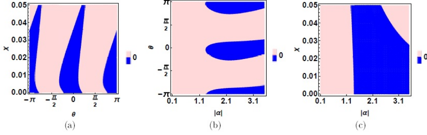
Figure 5.3: The dependence of HOS witness ( l = 4 ) on Kerr parameter \chi and displacement parameters |\alpha| and \theta for PAKS with (a) |\alpha| = 3 , (b) \chi = 0.02 , (c) \theta = 0 .
