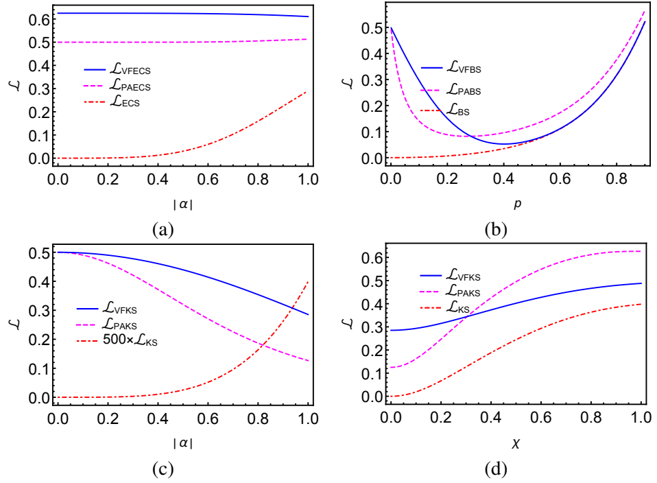
Figure 5.5: Illustration of linear entropy for (a) ECS, PAECS and VF ECS, (b) BS, PABS and VFBS, (c) KS, PAKS and VF KS with \alpha or p for \chi = 0.02 . (d) Dependence of nonclassicality in KS, PAKS and VF KS on \chi for \alpha = 1 .
